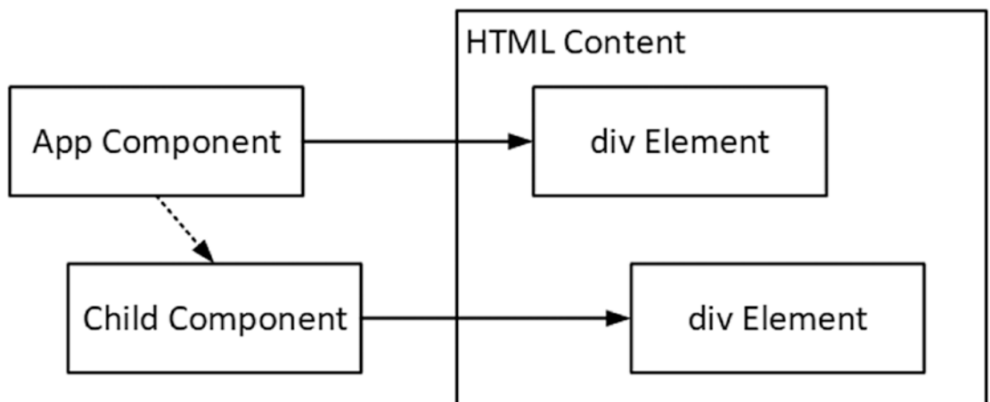
Figure 16-3. The parent-child component relationship
