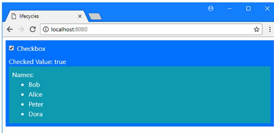
Figure 17-2. Accessing the DOM during the mounting lifecycle phase
