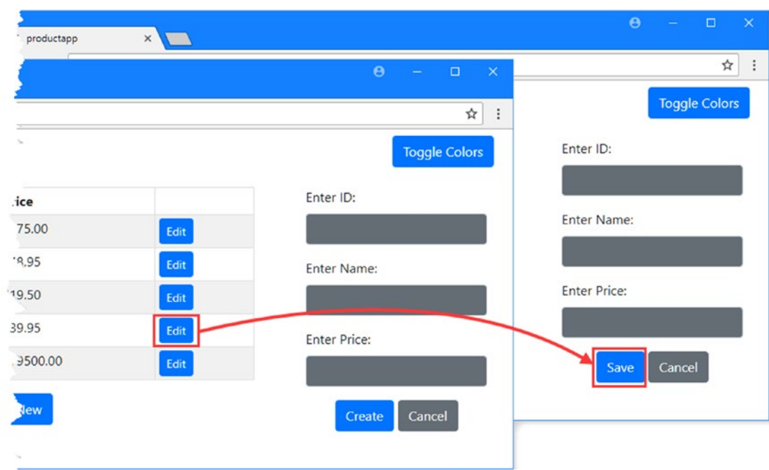
Figure 18-7. Using an event bus
