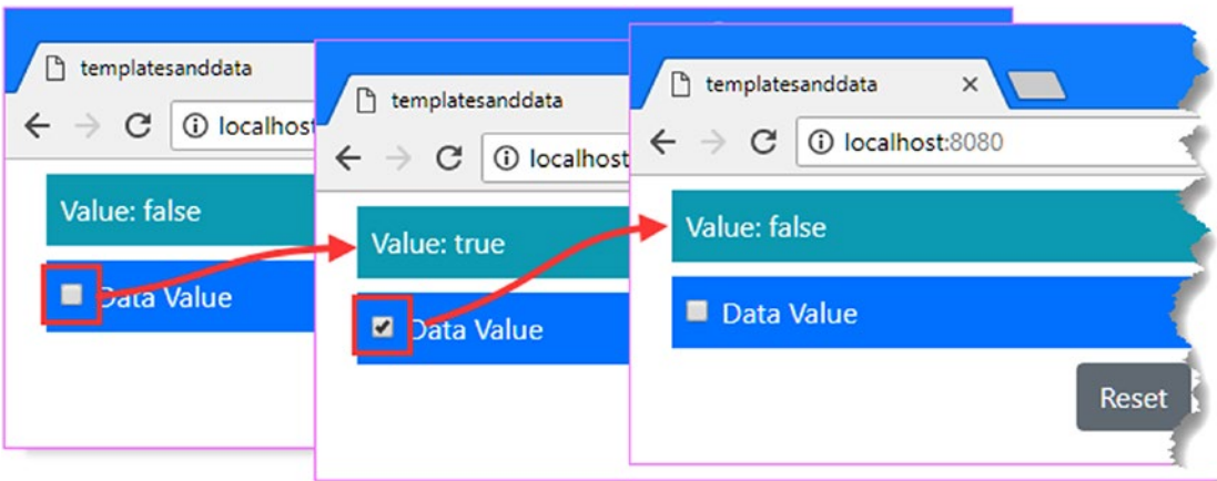
Figure 15-2. Using a one-way data binding
