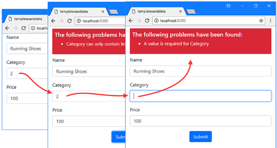
Figure 15-17. Immediate feedback for validation errors
